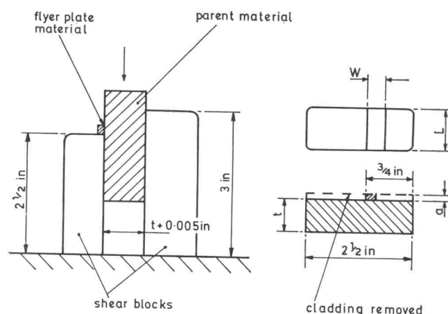
28 Shear tests on clad plate. Test-specimens: t > 2W ; W = \frac{1}{2}a . in 0.005 \frac{3}{4} 2\frac{1}{2} 3 mm 0.127 19.1 63.5 76.2
