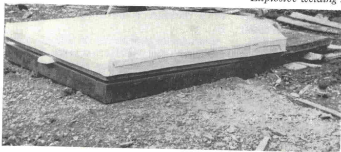
25 Arrangement for explosive cladding [3 ft-(1 m) square steel base with \frac{1}{2} in-(12.7 mm) thick aluminium bronze.]
